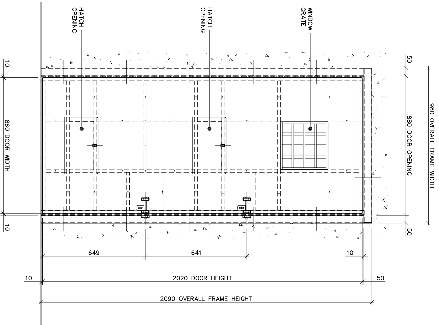
CELL DOOR ARRANGEMENT VIEWED ON OUTSIDE
