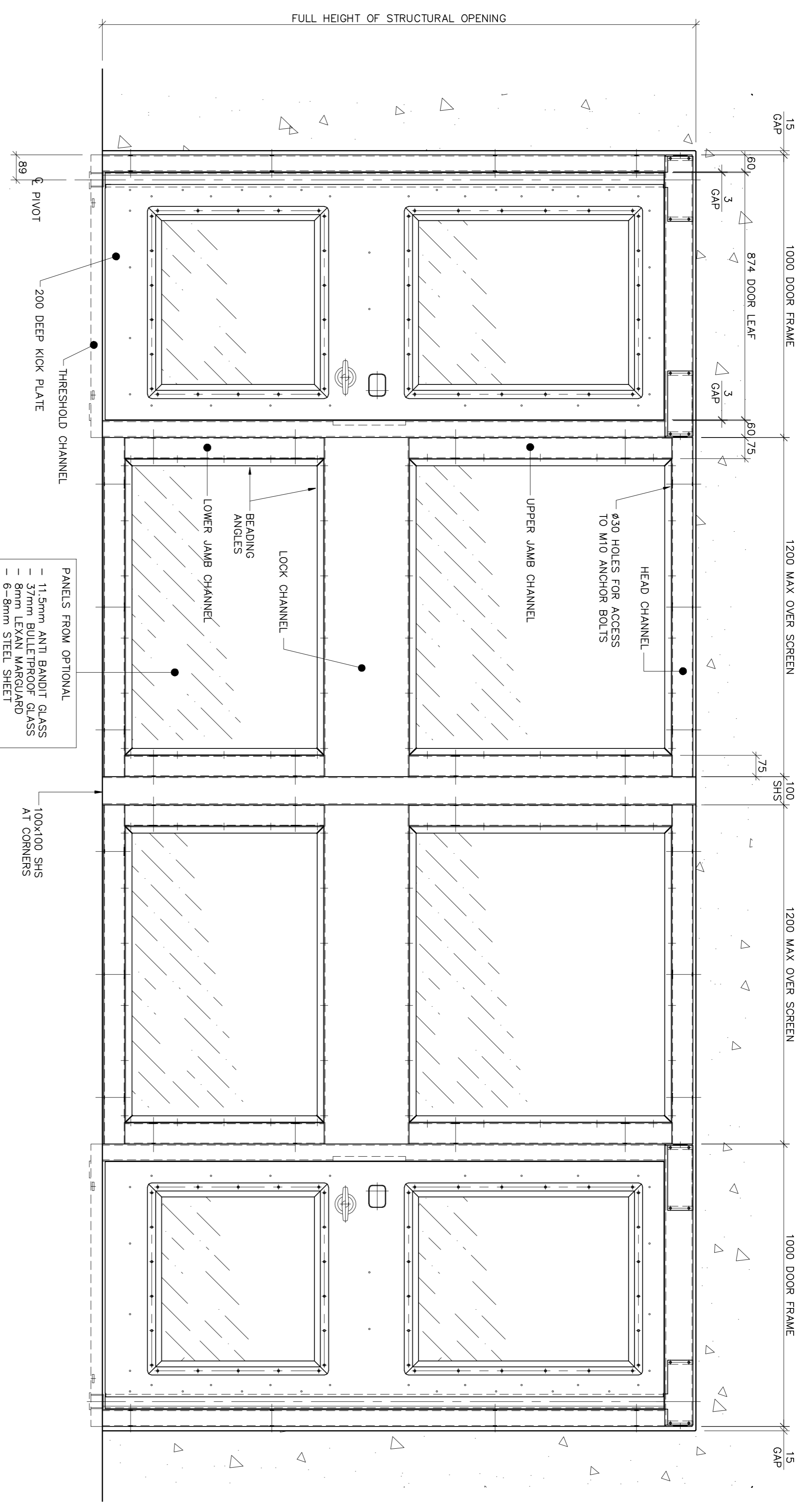
VIEW ON A-A - TYPICAL DOOR AND SCREEN ARRANGEMENT VIEWED ON SAFE SIDE
