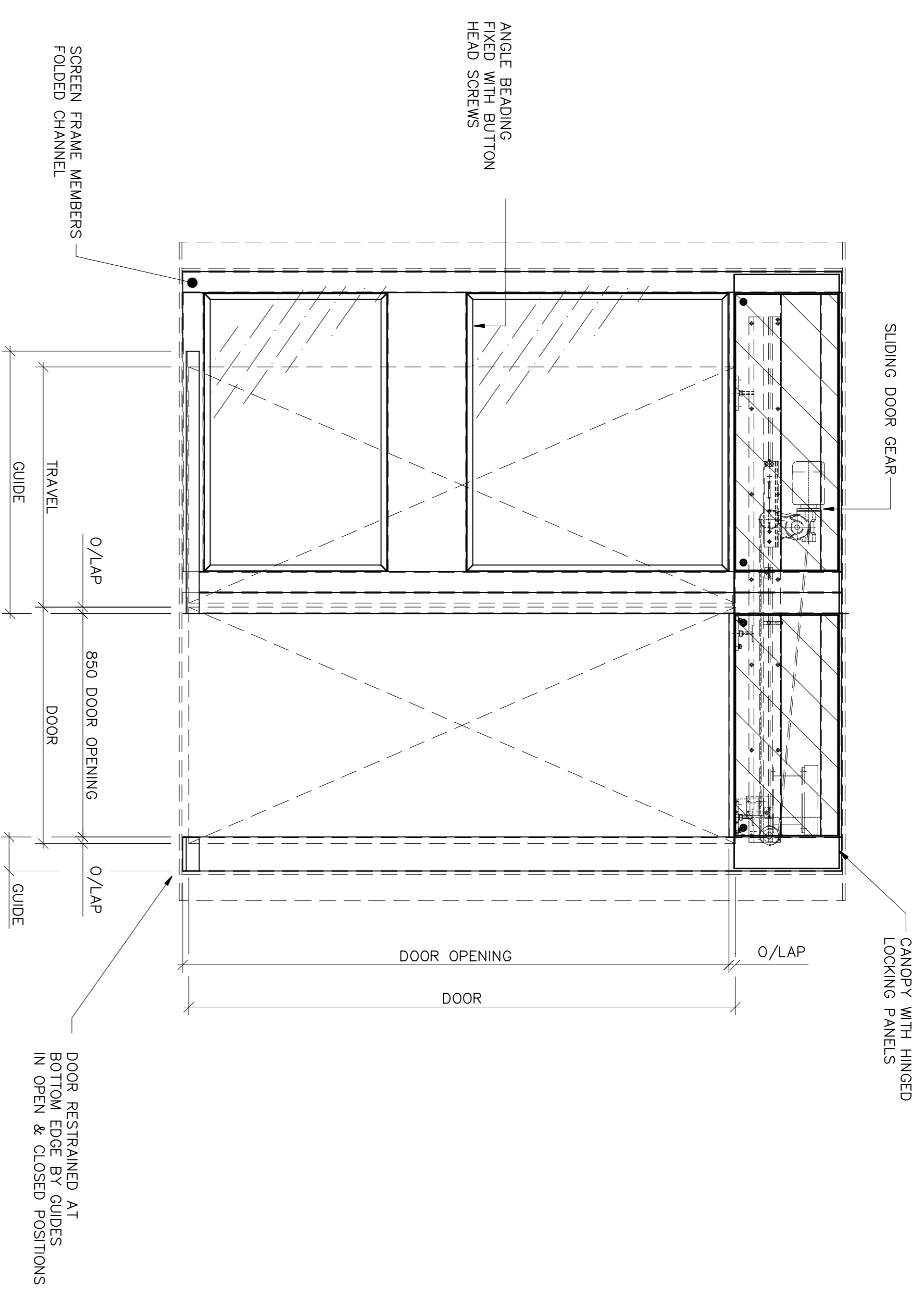
SCREEN ASSEMBLY VIEW ON SAFETY FACE DOOR SHOWN FAINT FOR CLARITY
