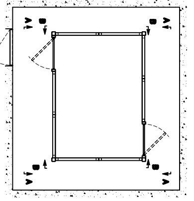
OPTION 3 - STAND ALONE CELL SCALE 1:15.000
