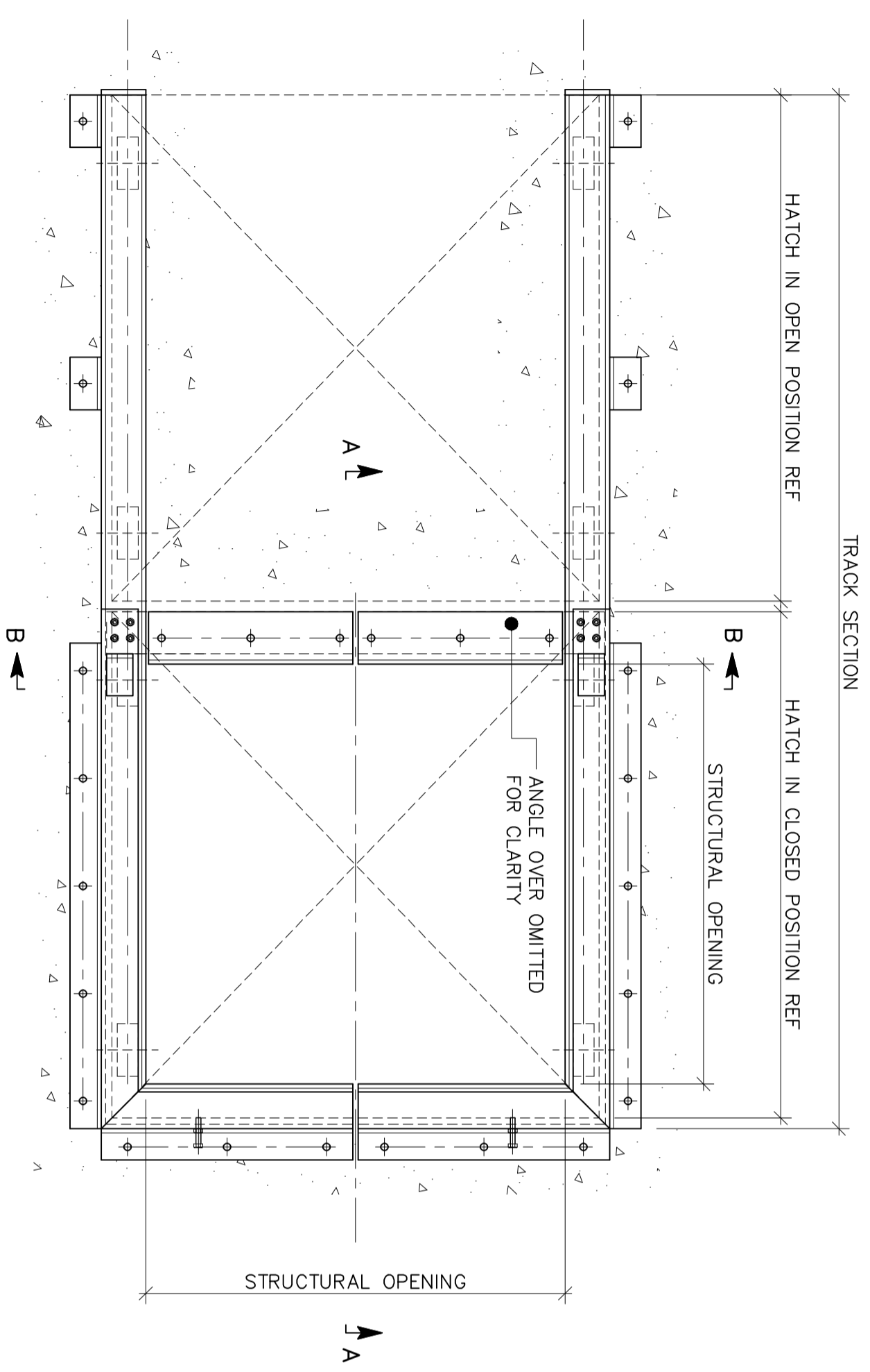
PLAN VIEW ON SECURITY HATCH FRAME
